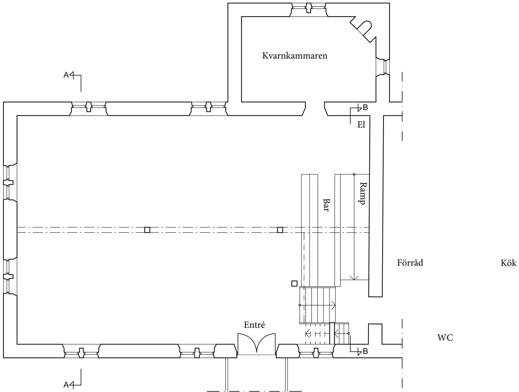
Plan BV, skala 1:100 (A4)
