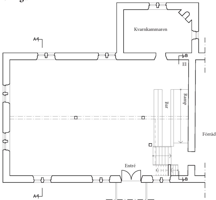
Plan BV, skala 1:100 (A4)
