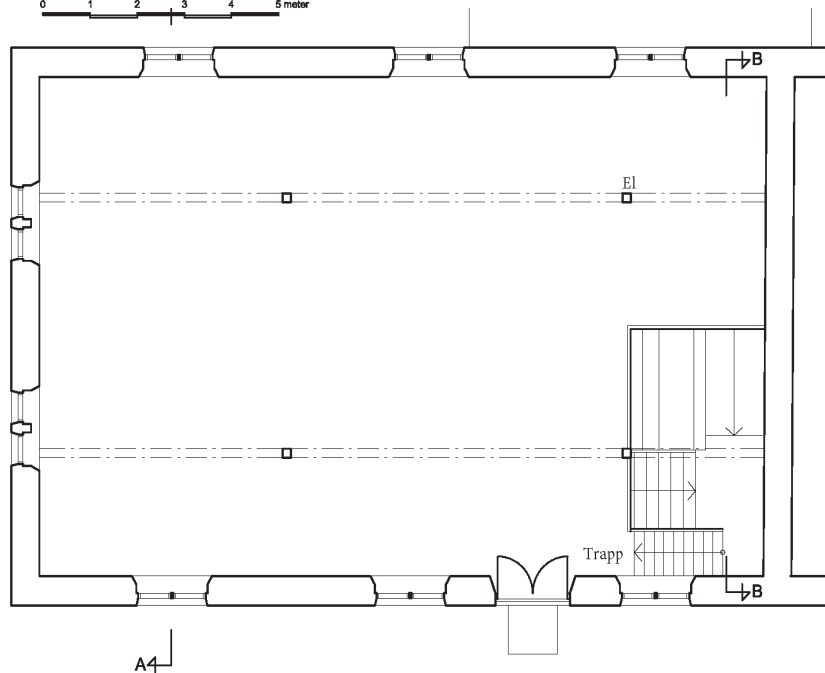
Plan BV, skala 1:100 (A4)
